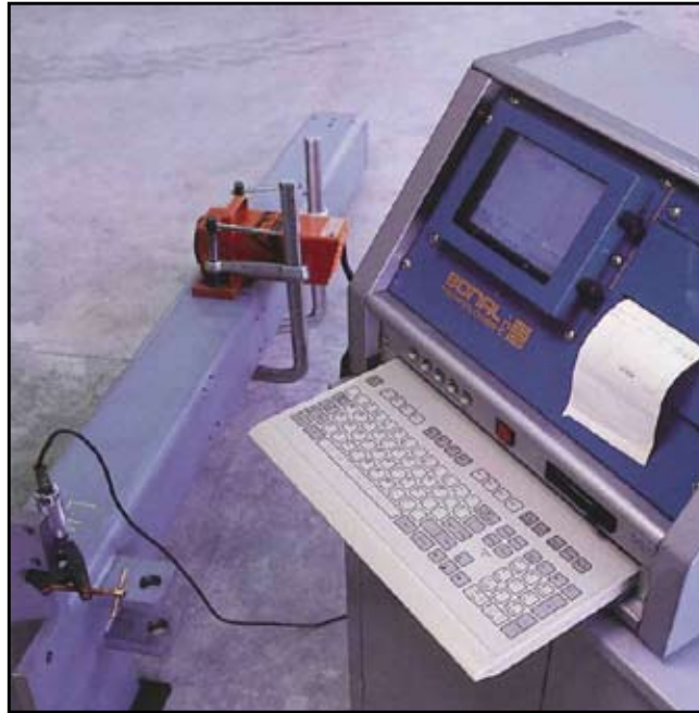
The Meta-Lax process performed on a support beam.
